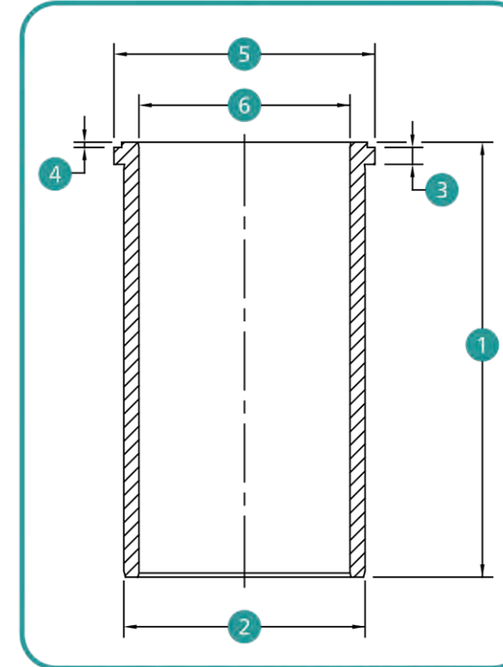
DRY TYPE WITH FLANGE
