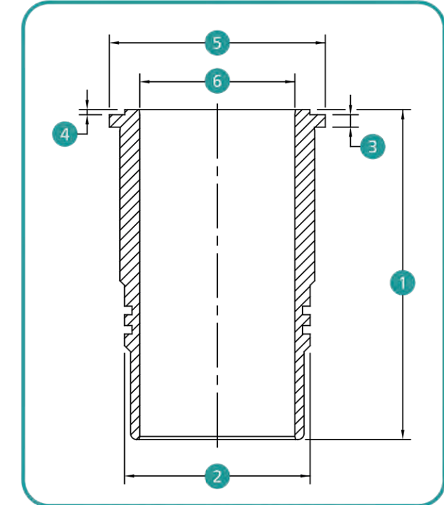
WET TYPE WITH FLANGE
